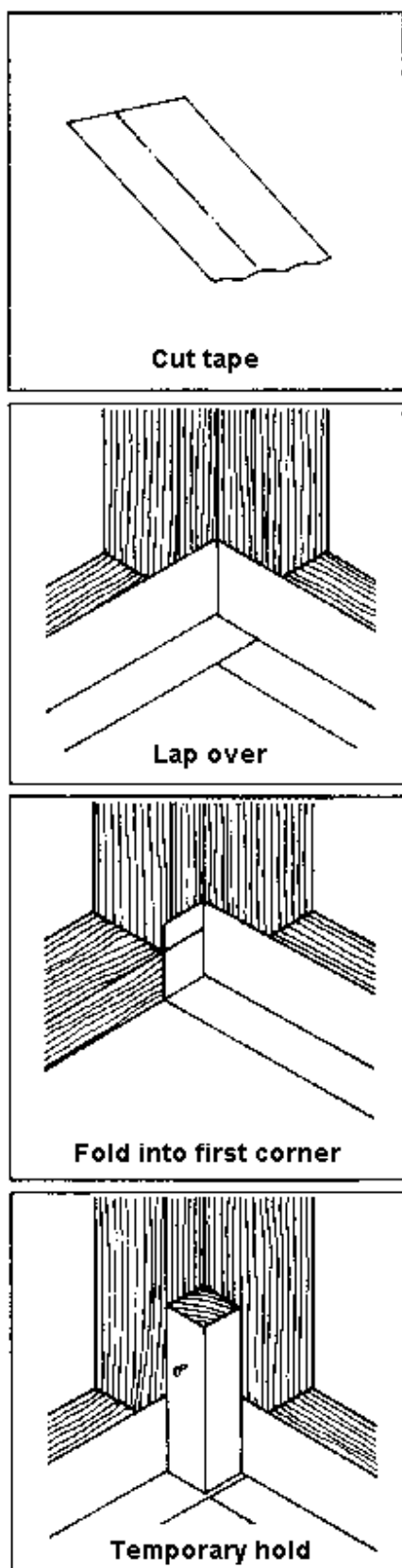
Figure 9 Corner Flashing for Showers
