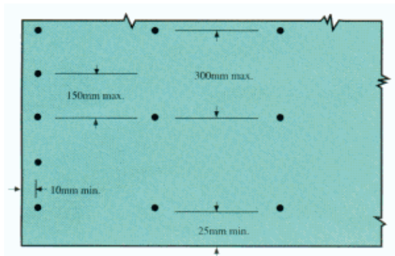
Figure 5 Standard Fixing
