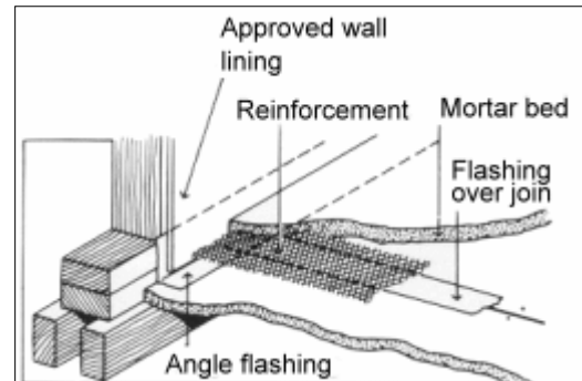
Figure 8 Room Perimeter Detail
