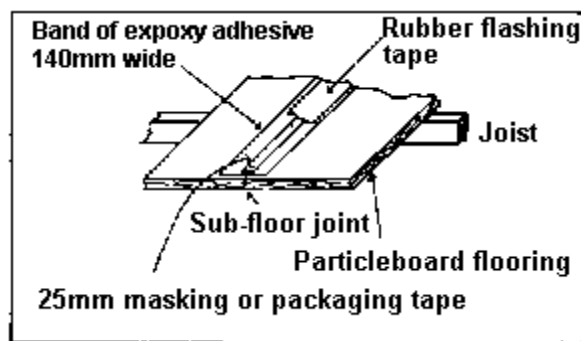
Figure 9 Butt Joint Detail
