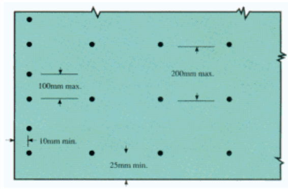
Figure 6 Close Fixing
