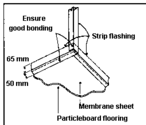
Figure 10 Flexible Membrane Shower Base
