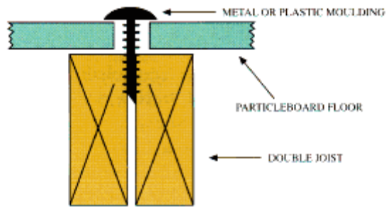
Figure 4 Expansion Joint.
