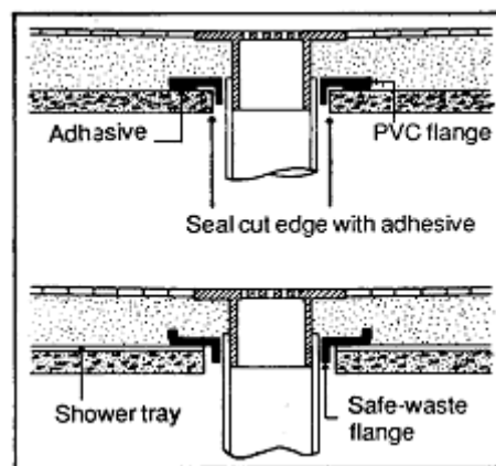
Figure 11 Floor Waste Installation
