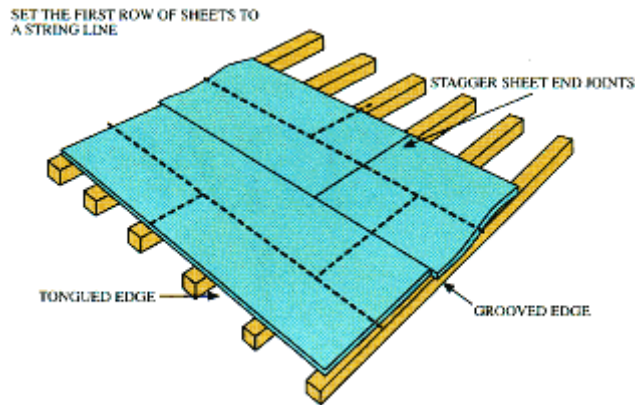
Figure 7 Double Layer Layout
