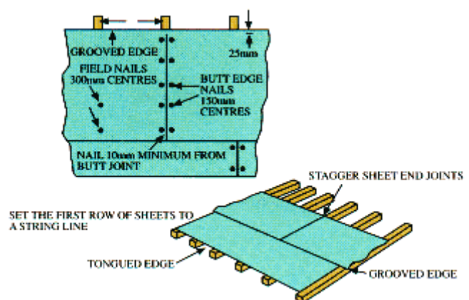
Figure 3 Sheet layout illustrating standard fixing.
