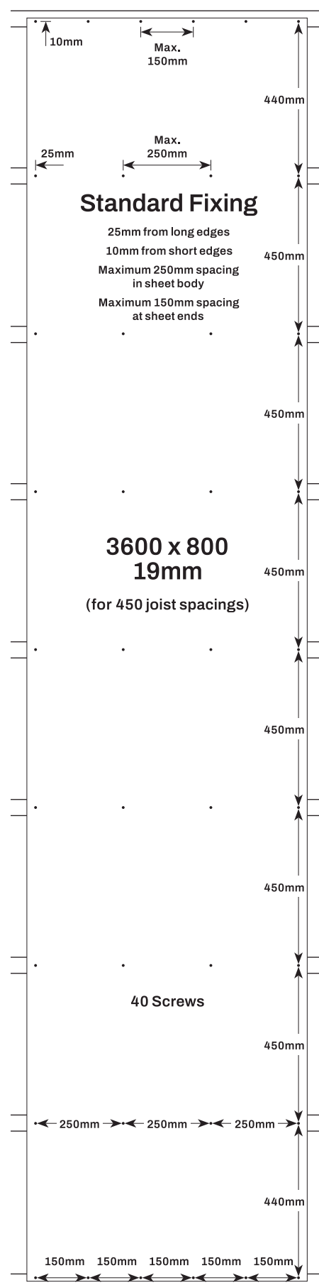
Figure 3. Fixing plan for 450mm joist spacing.
