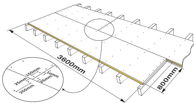
Figure 1 - Staggered Fixing
